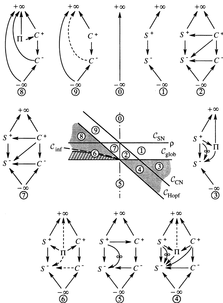
Figure 14. Schematic summary of connecting orbits for equation (2.14), b > 0 ; (a) c < 0 ; (b) c > 0 .
